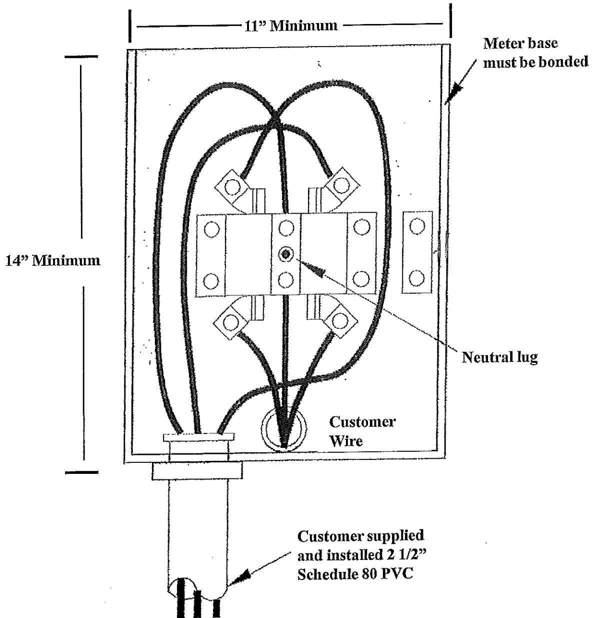
Figure D-2 200 Amp underground meter base
